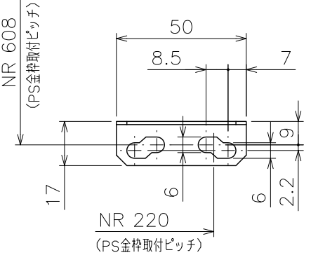
■I部詳細 (S=1/2)
